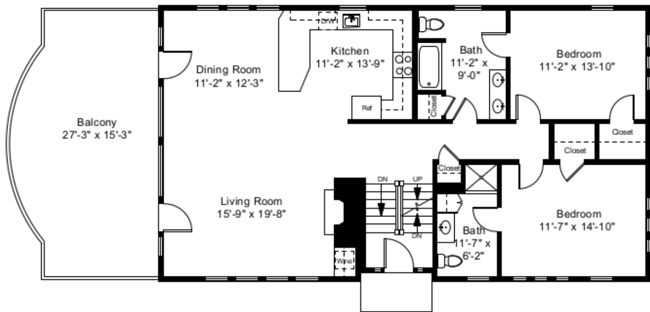
First Floor Plan Ceiling Height = 7'-11"
