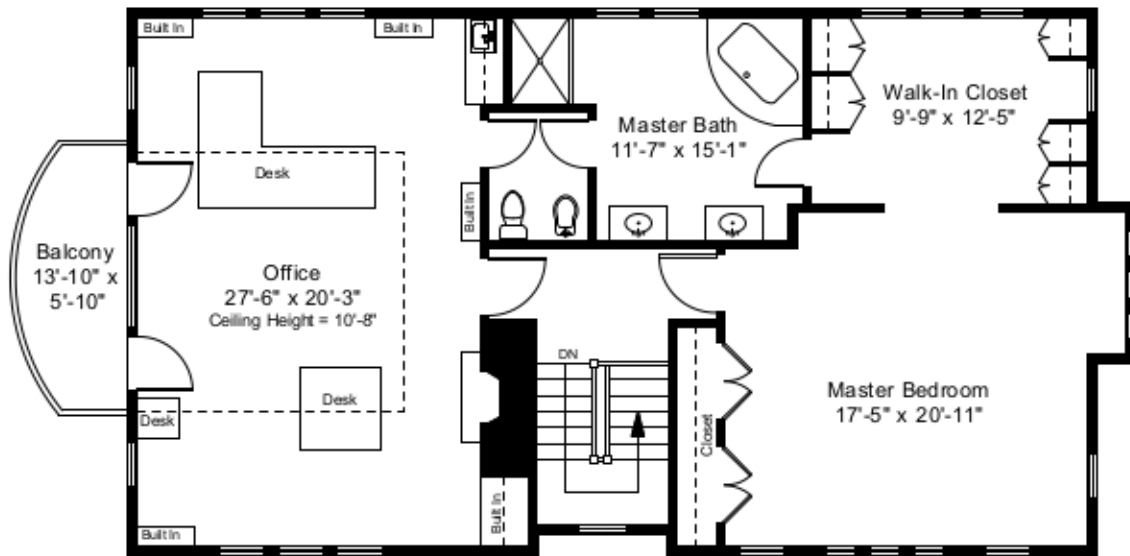
Second Floor Plan Ceiling Height = 7'-7"
